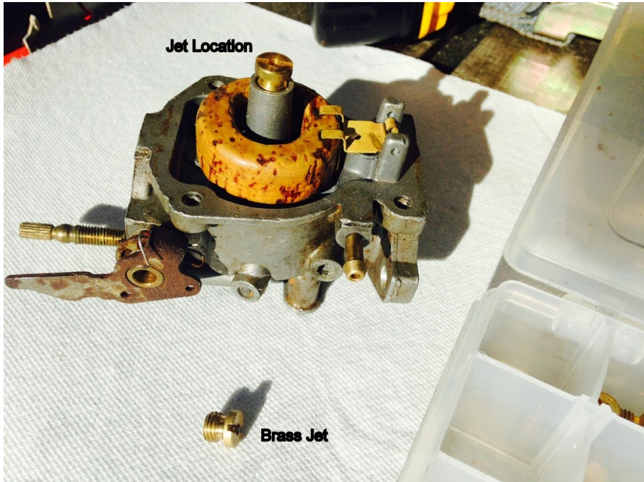
Figure 12. OMC A carb with float bowl removed. The brass jet is located on the top and another jet is shown on the workbench.
